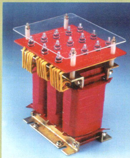
THREE PHASE AUTO TRANSFORMER
